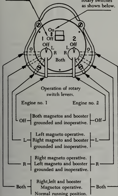
FIGURE 4-15. Magneto switch for a twin-engine aircraft.
